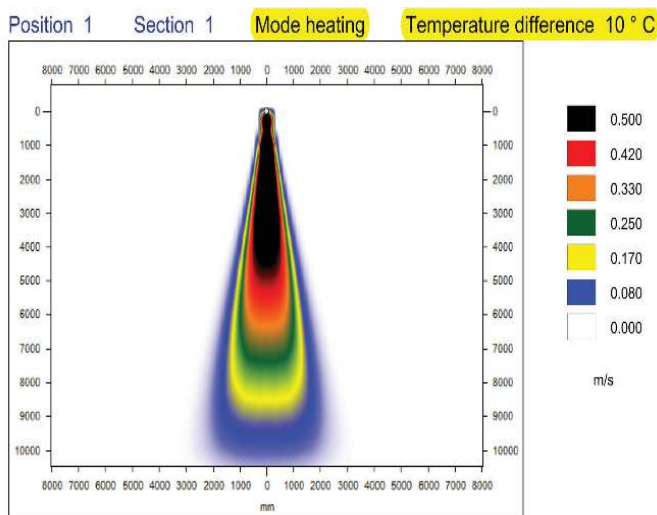
Prihoda Software Air Flow Graphic (Quote Specific)
